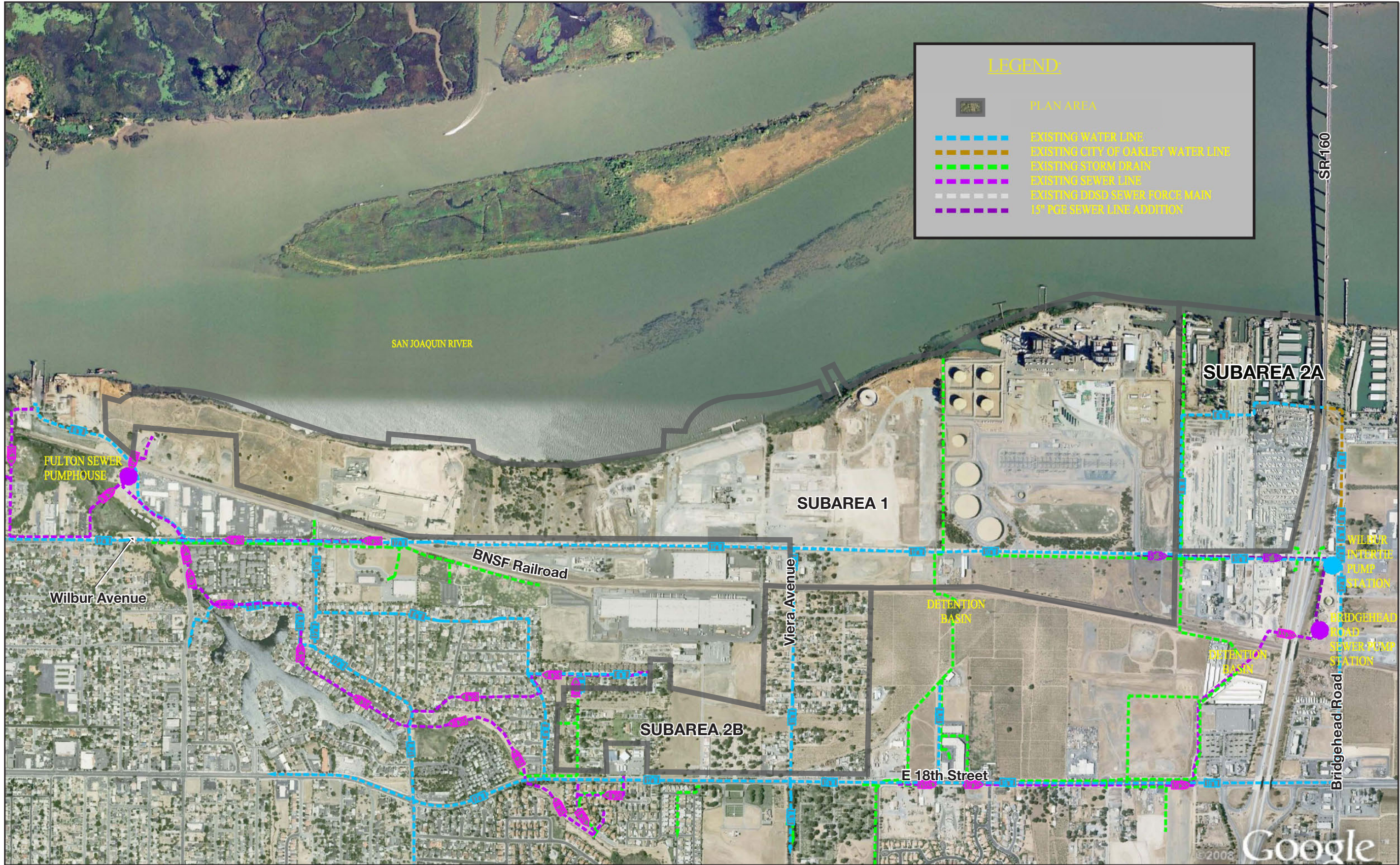
Existing Utilities Figure 6
