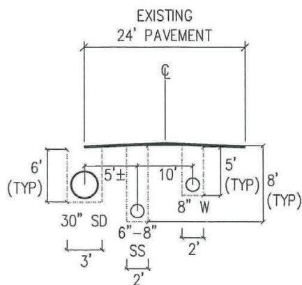
CROSS SECTION 3 BOWN LANE
