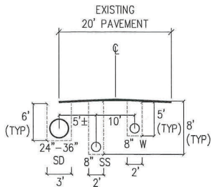
CROSS SECTION 2 SANTA FE AVE. WALNUT AVE.
