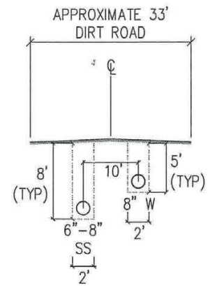
CROSS SECTION 4 TREMBATH LANE WYMORE WAY
