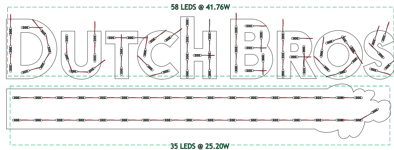
LED LAYOUT
