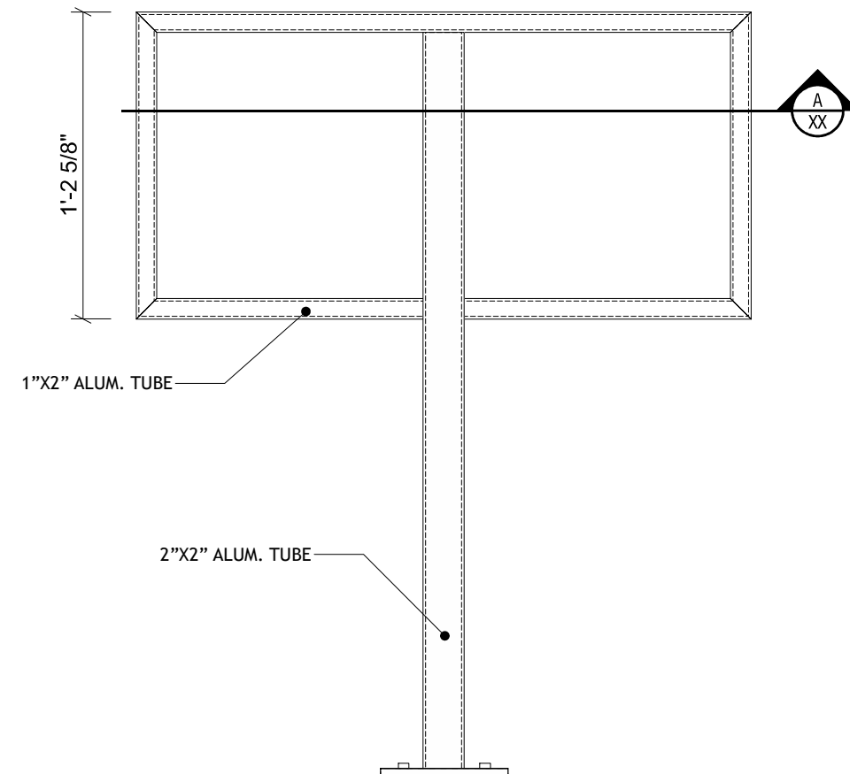
STRUCTURE DETAIL
