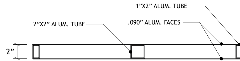
SECTION DETAIL
