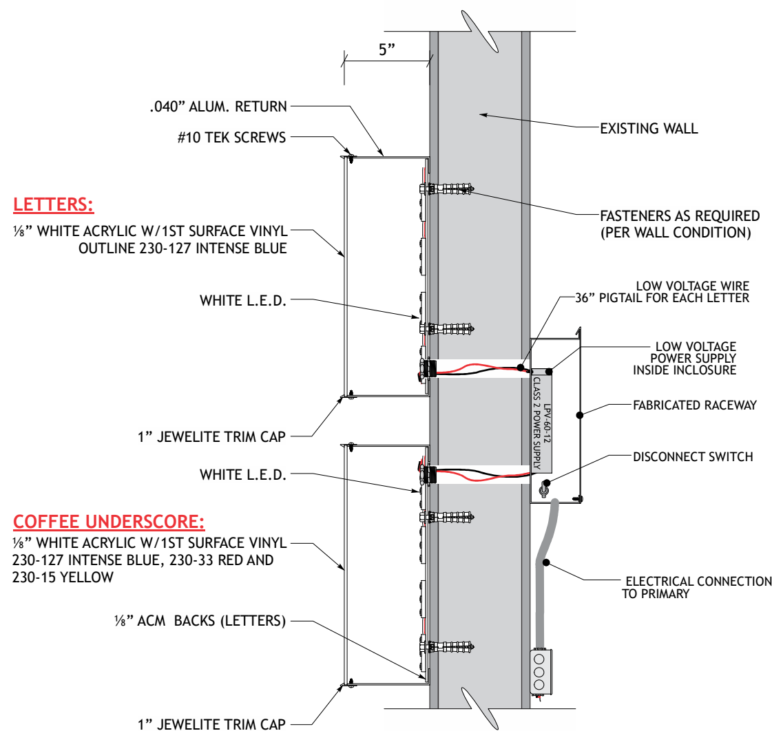
LED LAYOUT
